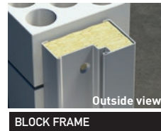
BLOCK FRAME
