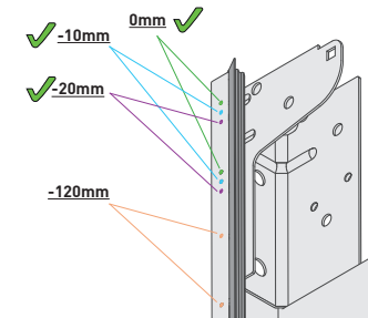
Between fix bracket shown from both sides on a no-hole frame leg.
