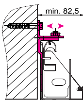
Between fix bracket shown from both sides on a no-hole frame leg.
